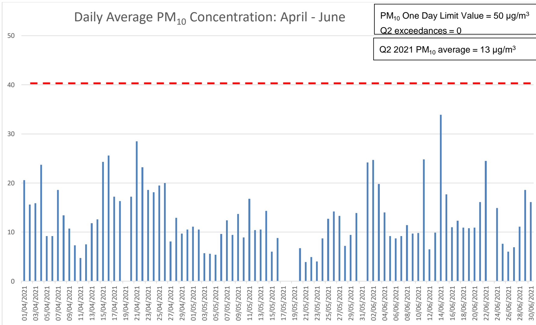
Figure 5 Daily Average PM 10 Q2 2021
