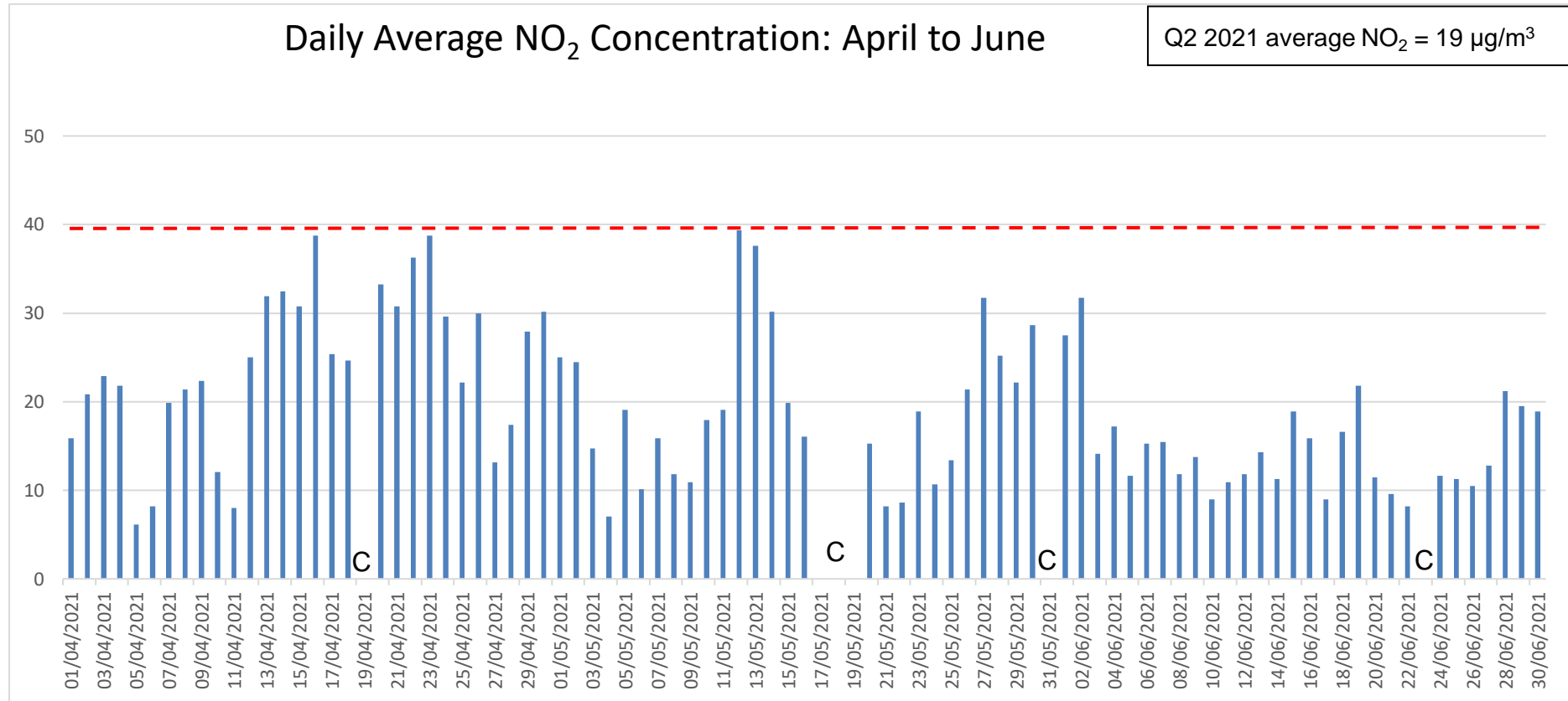
Figure 4 Daily Average NO 2 Q2 2021
