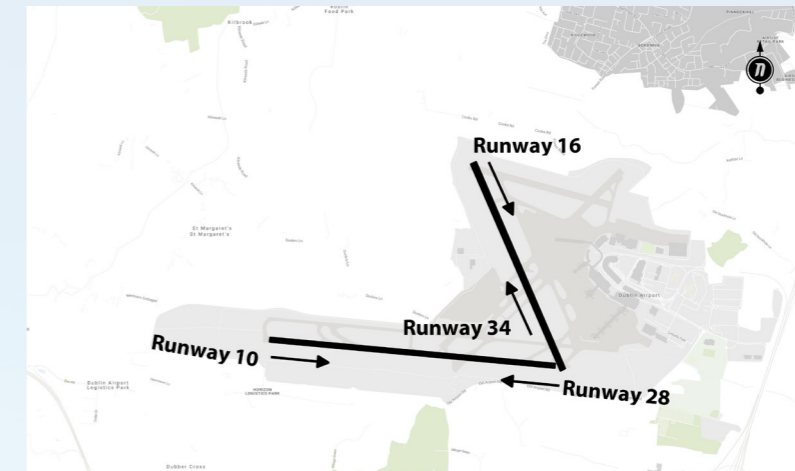
Figure 1: Runway layout Dublin Airport
