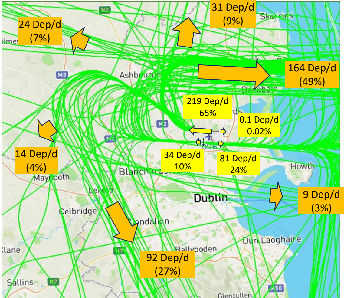
Graphic depicts: • Average departure movements per day on each main runway (yellow boxes) • % departures on each main runway for whole of 2024 (yellow boxes) • Average departures per day on each main track swathe (orange boxes) • Note: example flight track selection used
