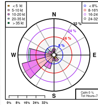
Windrose Dublin Apt December 2024
