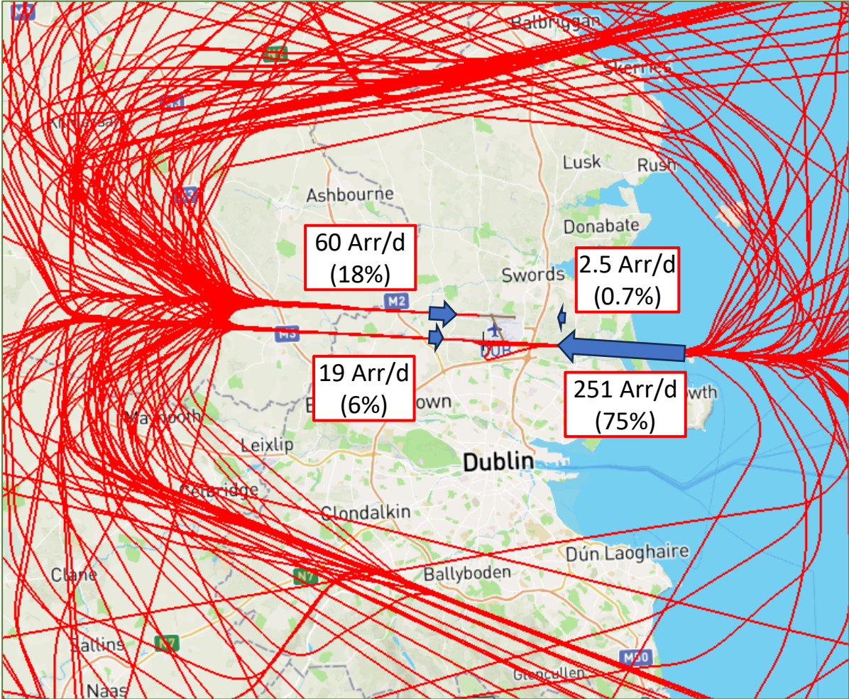
Graphic depicts: • Average arrival movements per day (d) on each main runway • % arrivals on each main runway for whole of 2024 • Note: example flight track selection used
